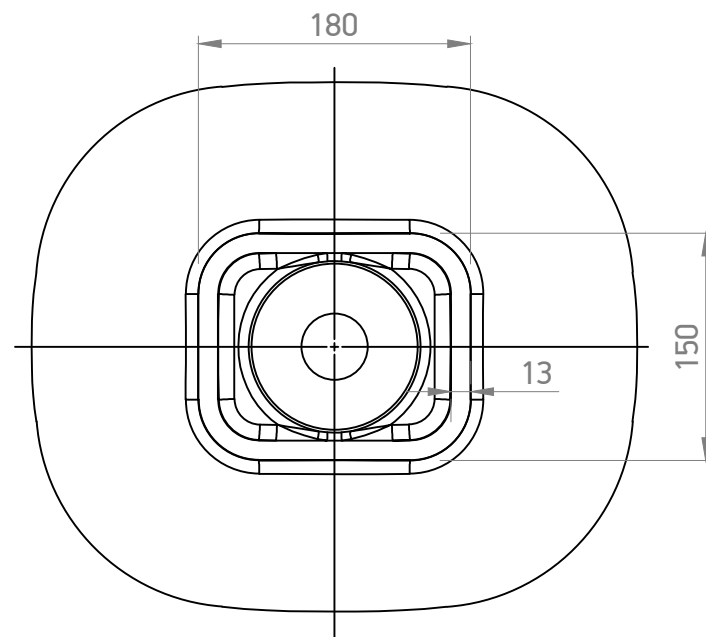
Bottom view
